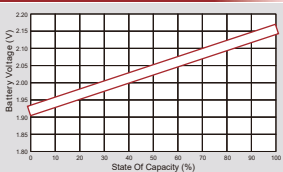
Relationship of OCV And State of Charge(20°C)
